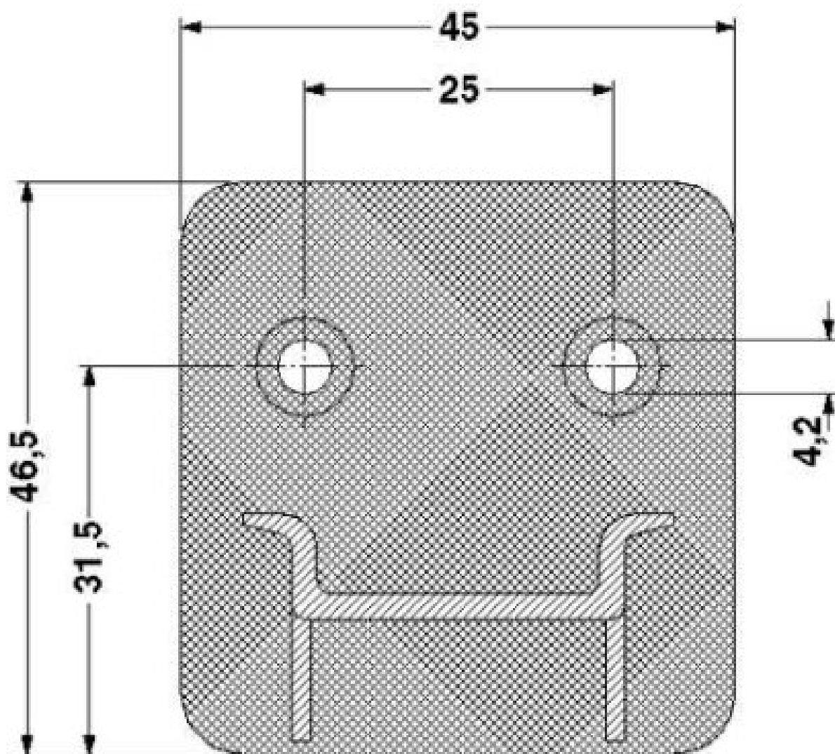
Dimensional drawing
